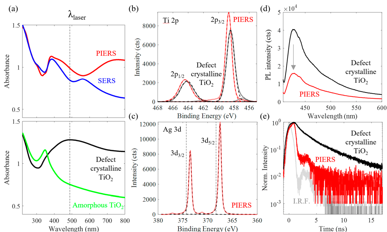
Figure 3. Charge transfer from \text{TiO}_2 oxygen vacancies to AgNPs. (a) Diffuse reflectance UV–vis spectra of (top) PIERS and SERS substrates; (bottom) defect crystalline \text{TiO}_2 (annealed at 600 °C in Ar for 1 h) and amorphous \text{TiO}_2 . The gray dotted line indicates the center wavelength of the Raman excitation laser (488 nm). (b) Ti 2p XPS of the PIERS and SERS substrates, with dotted lines indicating mixed Gaussian–Lorentzian fits to the 2p peaks for \text{Ti}^{4+} and \text{Ti}^{3+} . (c) Ag 3d XPS of PIERS substrate, where the vertical dotted lines are the standard binding energies of metallic Ag 56 and dotted lines indicating mixed Gaussian–Lorentzian fits to the 3d peaks. (d) Photoluminescence spectra of the PIERS substrate and defect crystalline \text{TiO}_2 (325 nm excitation laser, 1 mW). (e) Fluorescence decay lifetime at 460 nm of the PIERS substrate, defect crystalline \text{TiO}_2 , and instrument response function, I.R.F.
