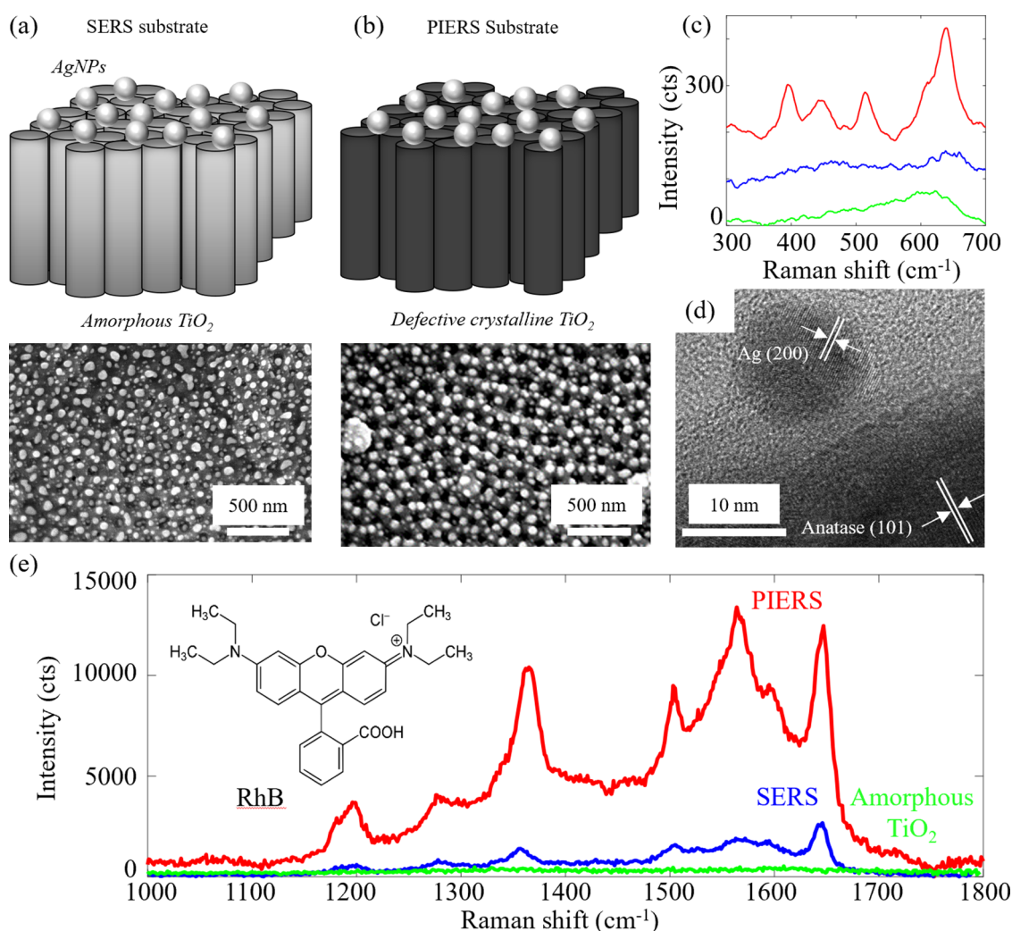
Figure 1. Enhanced Raman in PIERS substrates. (a) SEM image of SERS (Ag nanoparticles, AgNPs on amorphous \text{TiO}_2 ) substrate and (b) PIERS (AgNPs on crystalline defective \text{TiO}_2 , annealed at 600 °C for 1 h in Ar prior to AgNP formation) substrate with schematics above. (c) Raman spectra of bare as-anodized \text{TiO}_2 substrate (green), SERS substrate (blue), and PIERS substrate (red) with crystalline anatase (395 ( B_{1g} ), 515 ( A_{1g} ), and 639 ( E_g ) \text{cm}^{-1} ) 16 and rutile peaks (446 ( E_g ) and 606 ( A_{1g} ) \text{cm}^{-1} ). (d) TEM image of PIERS substrate with lattice fringes and phase indicated (detail in Figure S7). (e) Raman spectrum of Rhodamine B (10 \mu\text{M} ) on a bare \text{TiO}_2 substrate, a SERS substrate (enhancement factor 3.4 \times 10^5 ), and a PIERS substrate (enhancement factor 2.3 \times 10^6 ) averaged over 10 locations on a sample.
